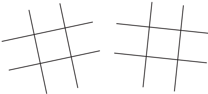
Tic-Tac-Toe
